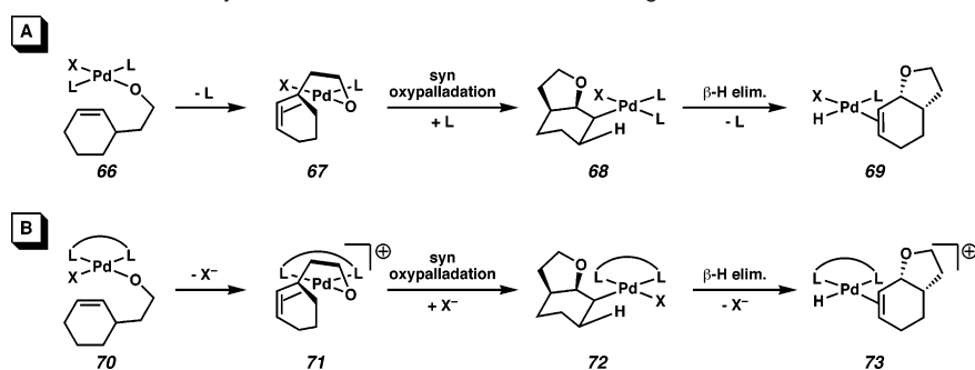
Scheme 6. Cyclization of Deuterium-Labeled Carboxylic Acid Substrates with Pyridine as Ligand
